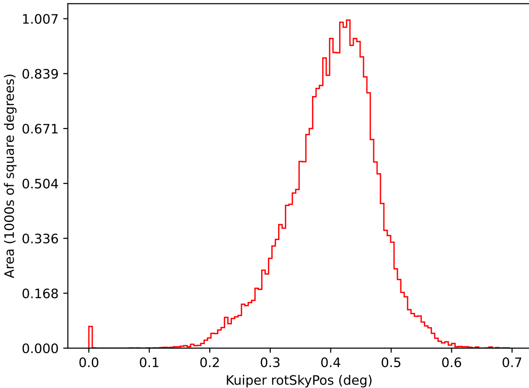
ddf_acor_sf20_lsf40_lsr20_v3.4_10yrs i: Kuiper rotSkyPos
