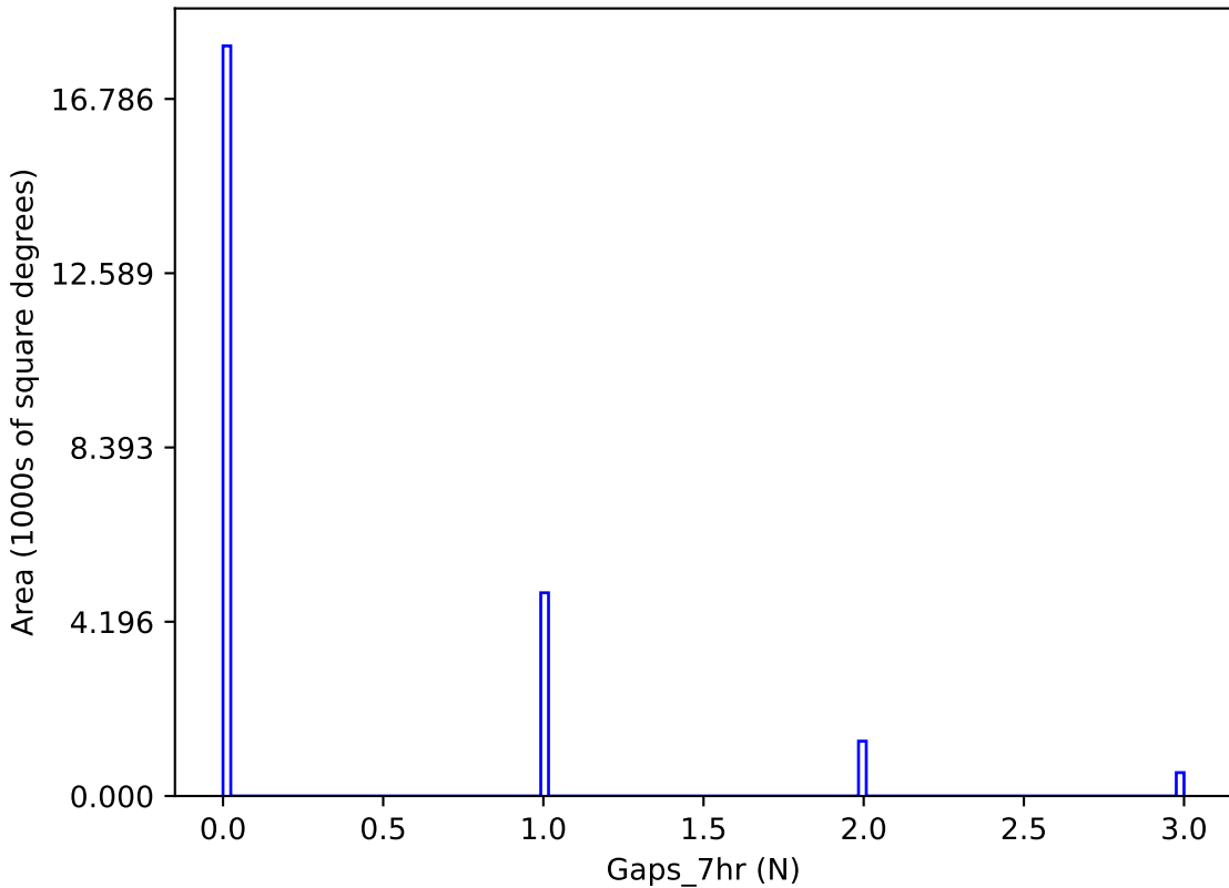
ddf_acor_sf20_lsf40_lsr20_v3.4_10yrs y band: Gaps_7hr
