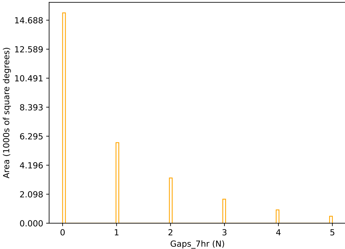
ddf_acor_sf20_lsf40_lsr20_v3.4_10yrs r band: Gaps_7hr
