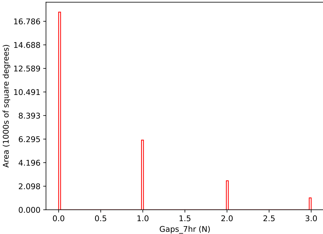
ddf_acor_sf20_lsf40_lsr20_v3.4_10yrs i band: Gaps_7hr
