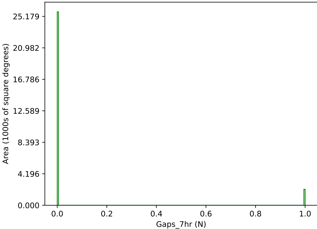
ddf_acor_sf20_lsf40_lsr20_v3.4_10yrs g band: Gaps_7hr
