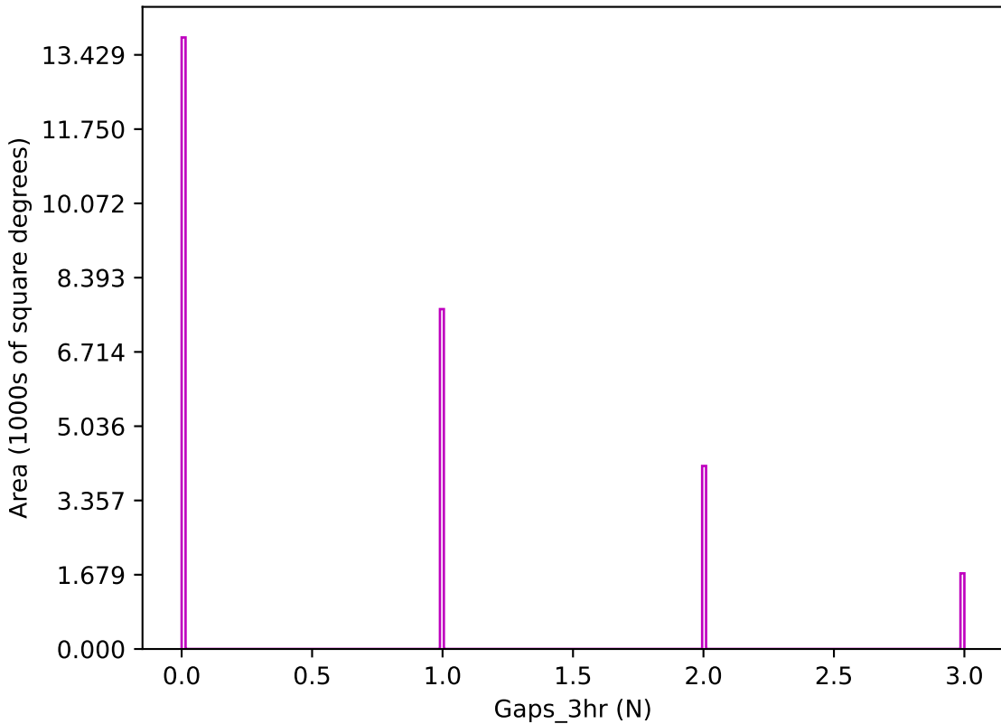
ddf_acor_sf20_ls40_lsr20_v3.4_10yrs z band: Gaps_3hr
