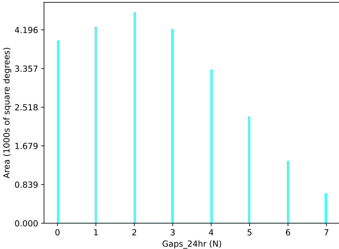
ddf_acor_sf20_lsf40_lsr20_v3.4_10yrs u band: Gaps_24hr
