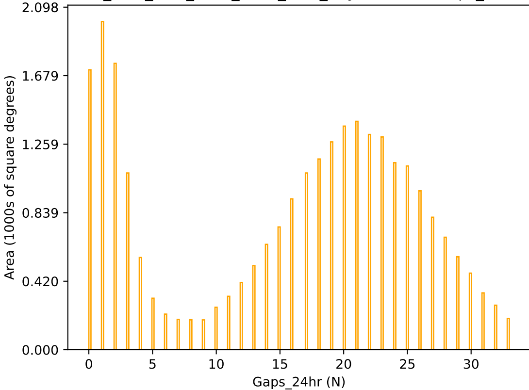
ddf_acor_sf20_lsf40_lsr20_v3.4_10yrs r band: Gaps_24hr
