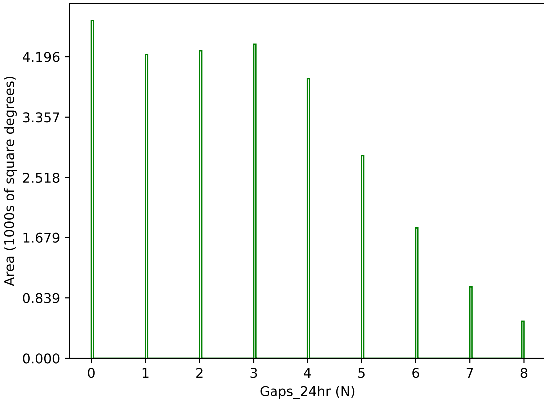
ddf_acor_sf20_lsf40_lsr20_v3.4_10yrs g band: Gaps_24hr
