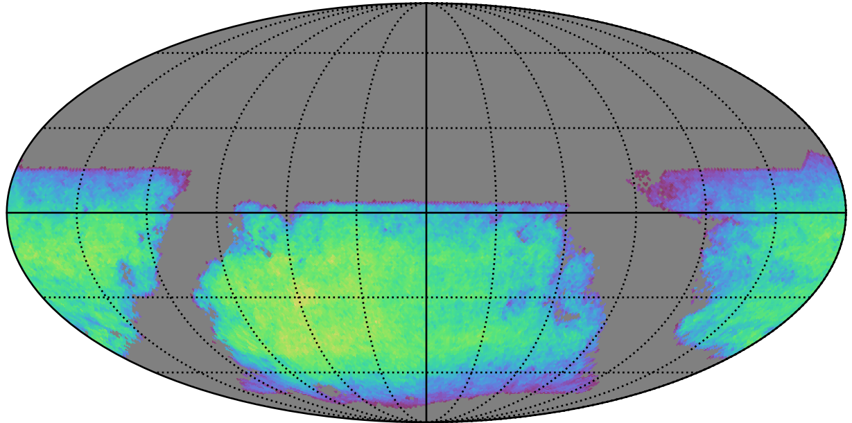
ddf_acor_sf20_lsf40_lsr20_v3.4_10yrs i band non-DD year 10: ExgalM5WithCuts
