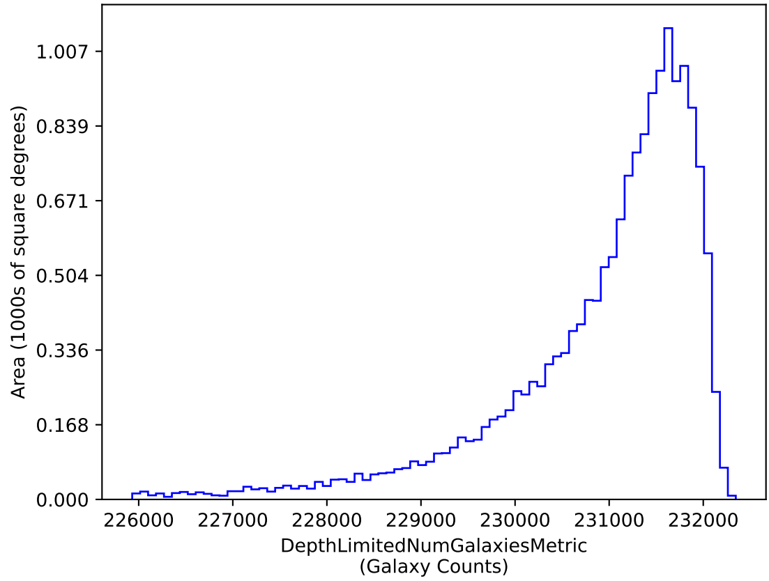
ddf_acor_sf20_lsf40_lsr20_v3.4_10yrs i band galaxies non-DD: DepthLimitedNumGalaxiesMetric
