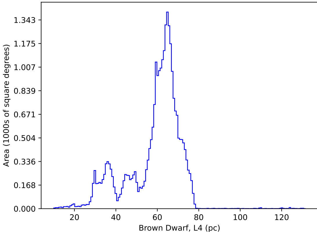
ddf_acor_sf20_lsf40_lsr20_v3.4_10yrs : Brown Dwarf, L4
