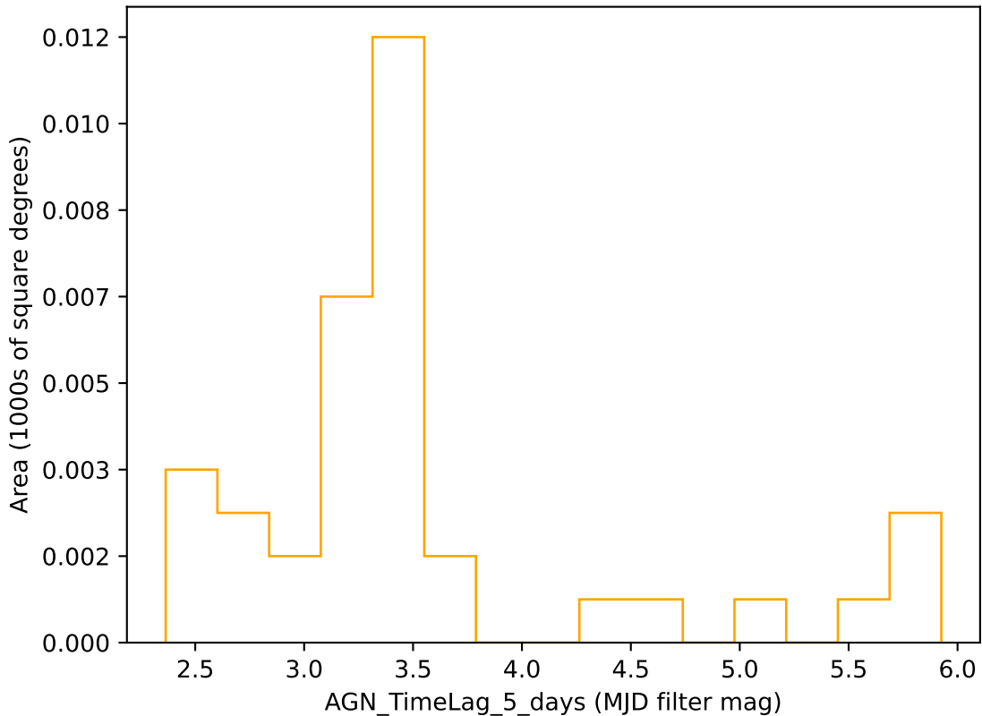
ddf_acor_sf20_lsf40_lsr20_v3.4_10yrs r band: AGN_TimeLag_5_days
