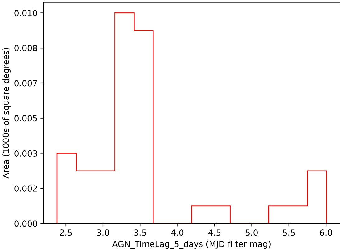
ddf_acor_sf20_lsf40_lsr20_v3.4_10yrs i band: AGN_TimeLag_5_days
