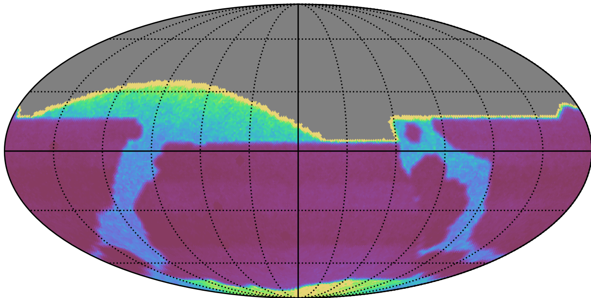
ddf_acor_sf20_lsf40_lsr20_v3.4_10yrs : properMotion
