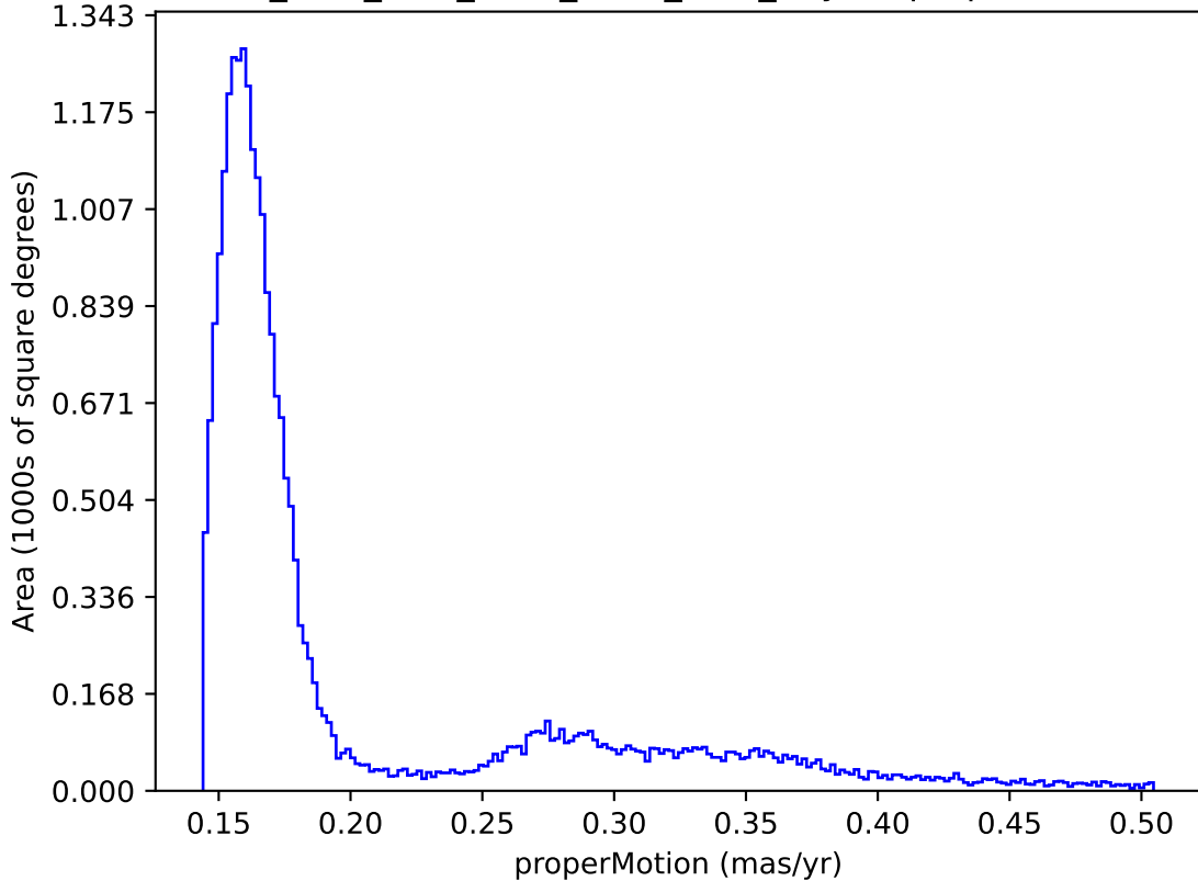
ddf_acor_sf20_lsf40_lsr20_v3.4_10yrs : properMotion
