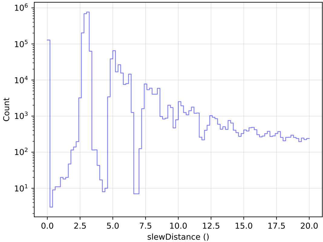
ddf_acor_sf20_lsf40_lsr20_v3.4_10yrs All visits: Zoom Slew Distance Histogram
