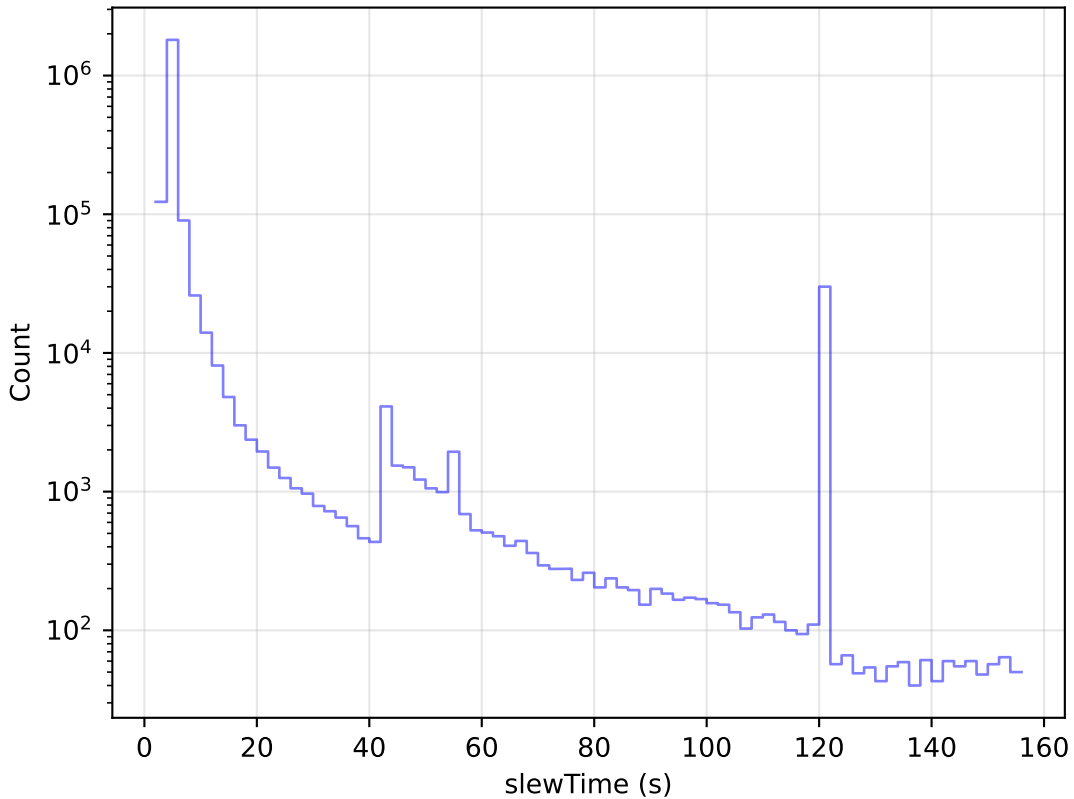
ddf_acor_sf20_lsf40_lsr20_v3.4_10yrs All visits: Slew Time Histogram
