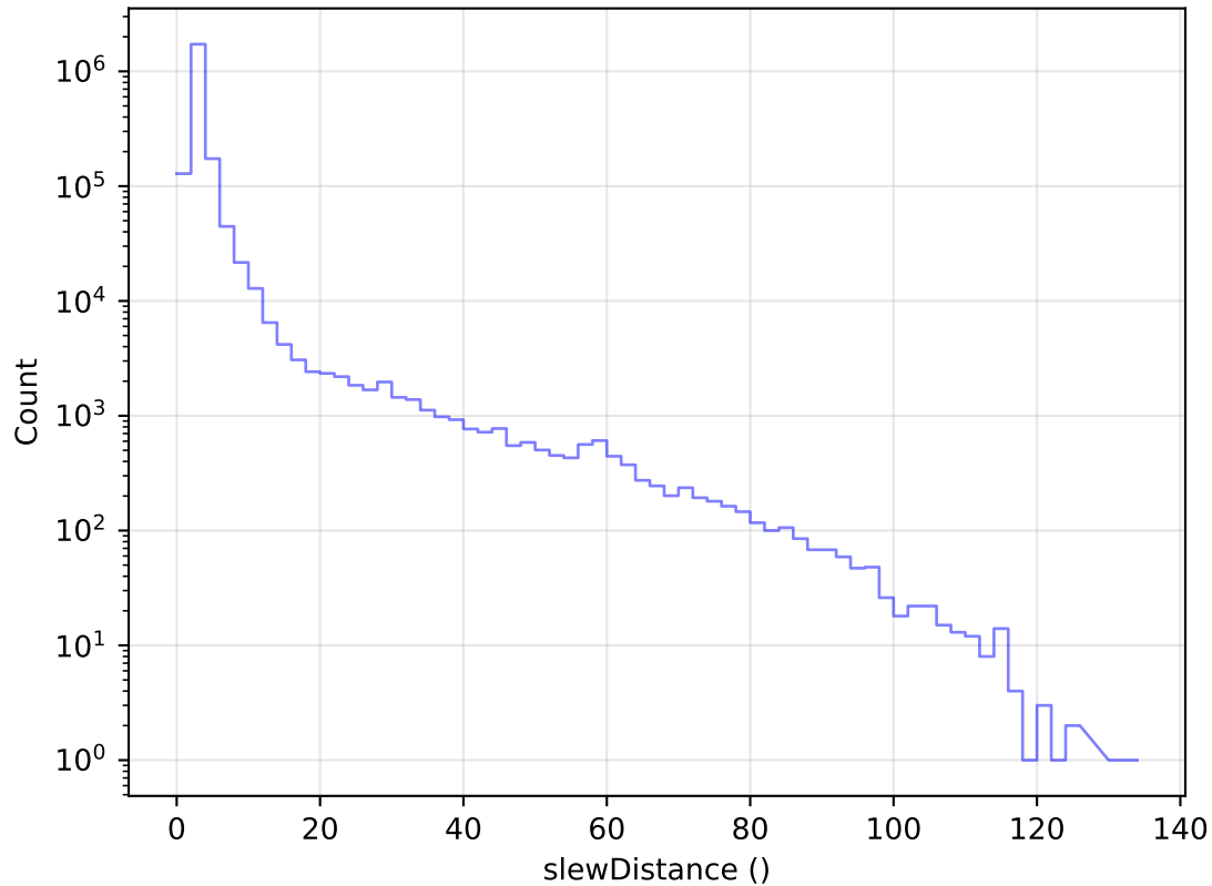
ddf_acor_sf20_lsf40_lsr20_v3.4_10yrs All visits: Slew Distance Histogram
