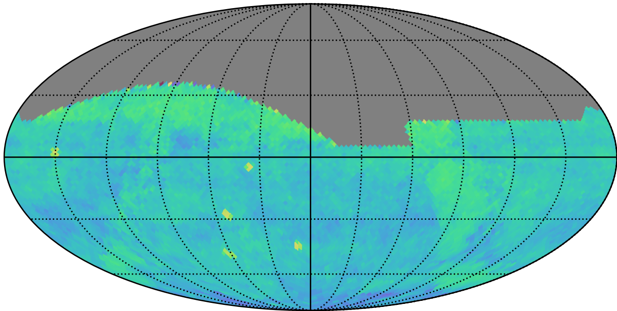
ddf_acor_sf20_lsf40_lsr20_v3.4_10yrs (g or r or i): PairFraction
