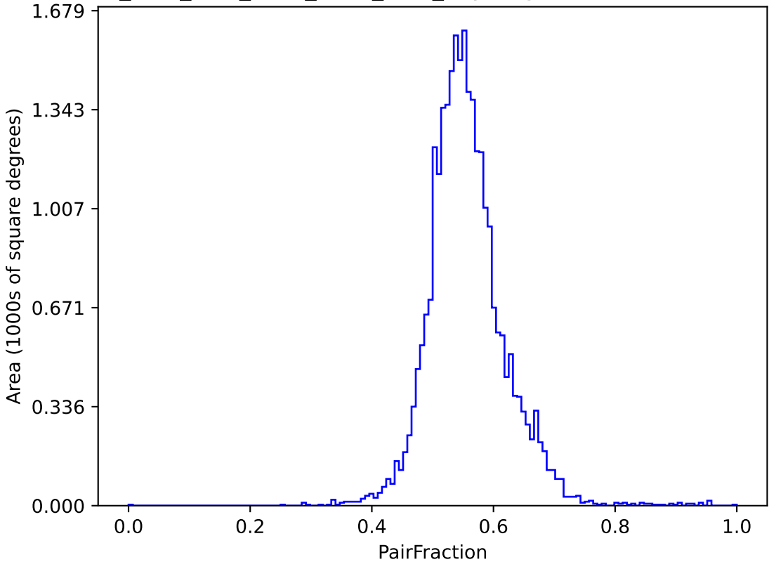
ddf_acor_sf20_lsf40_lsr20_v3.4_10yrs (g or r or i): PairFraction
