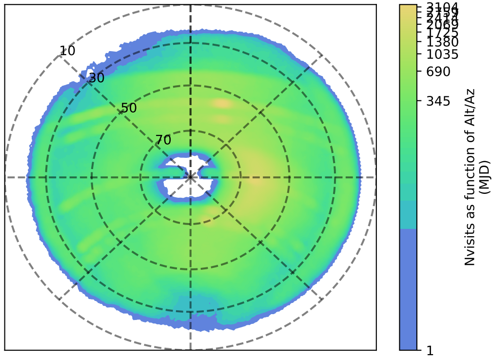
ddf_acor_sf20_lsf40_lsr20_v3.4_10yrs z: Nvisits as function of Alt/Az
