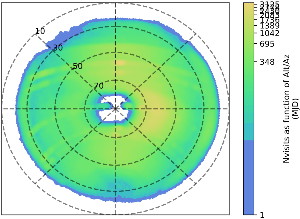
ddf_acor_sf20_lsf40_lsr20_v3.4_10yrs i: Nvisits as function of Alt/Az
