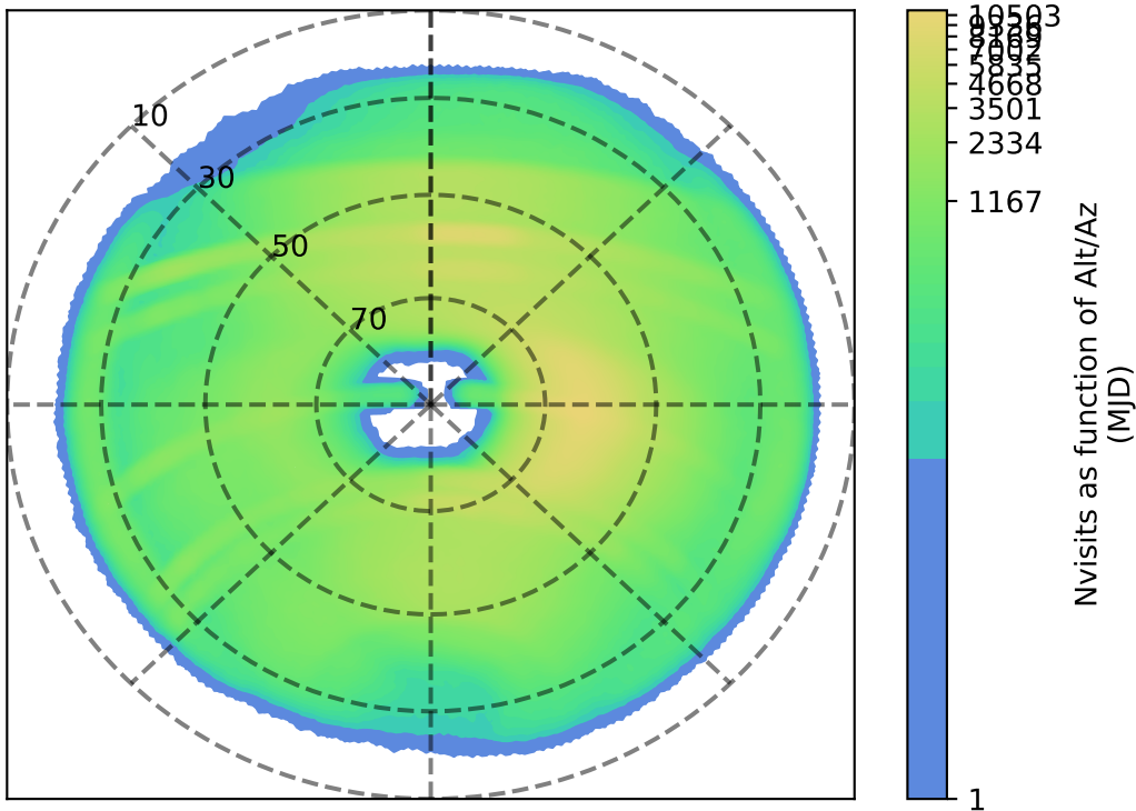
ddf_acor_sf20_lsf40_lsr20_v3.4_10yrs : Nvisits as function of Alt/Az
