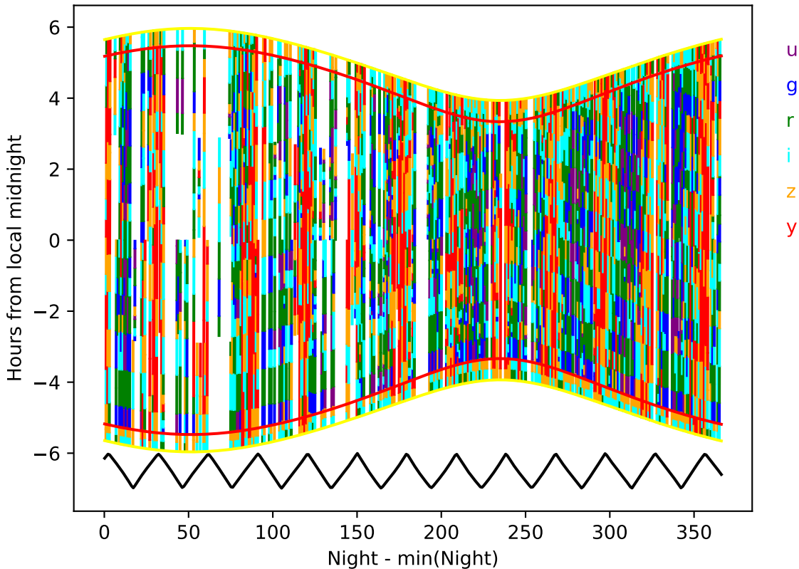
ddf_acor_sf20_lsf40_lsr20_v3.4_10yrs year 9-10: Hourglass
