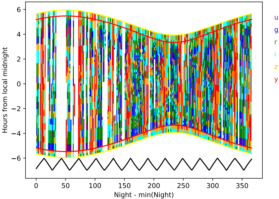
ddf_acor_sf20_lsf40_lsr20_v3.4_10yrs year 8-9: Hourglass
