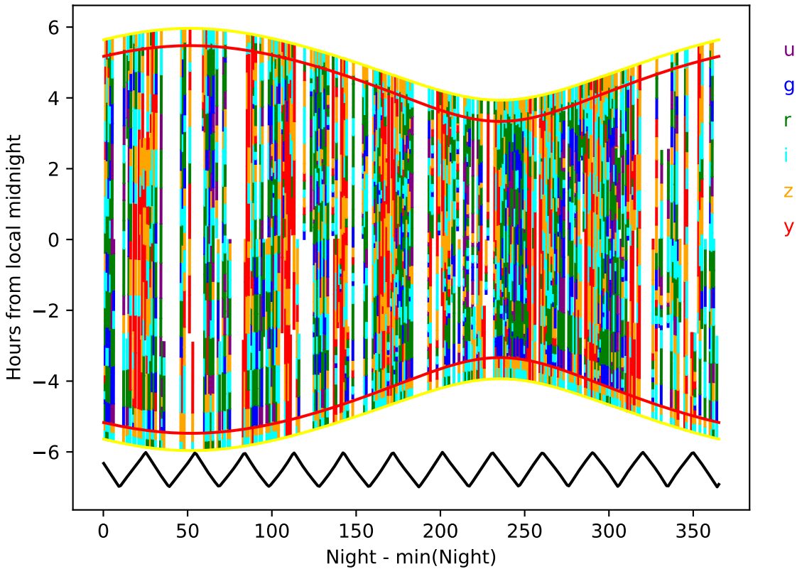
ddf_acor_sf20_lsf40_lsr20_v3.4_10yrs year 7-8: Hourglass
