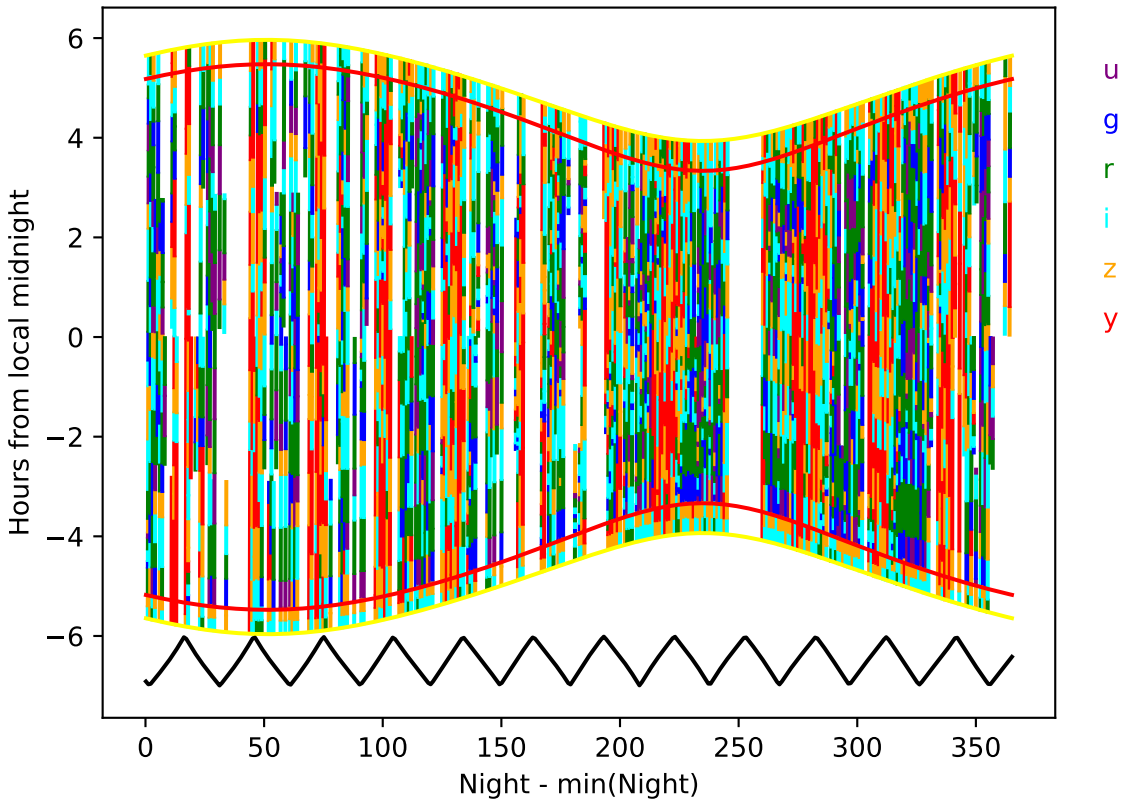
ddf_acor_sf20_lsf40_lsr20_v3.4_10yrs year 5-6: Hourglass
