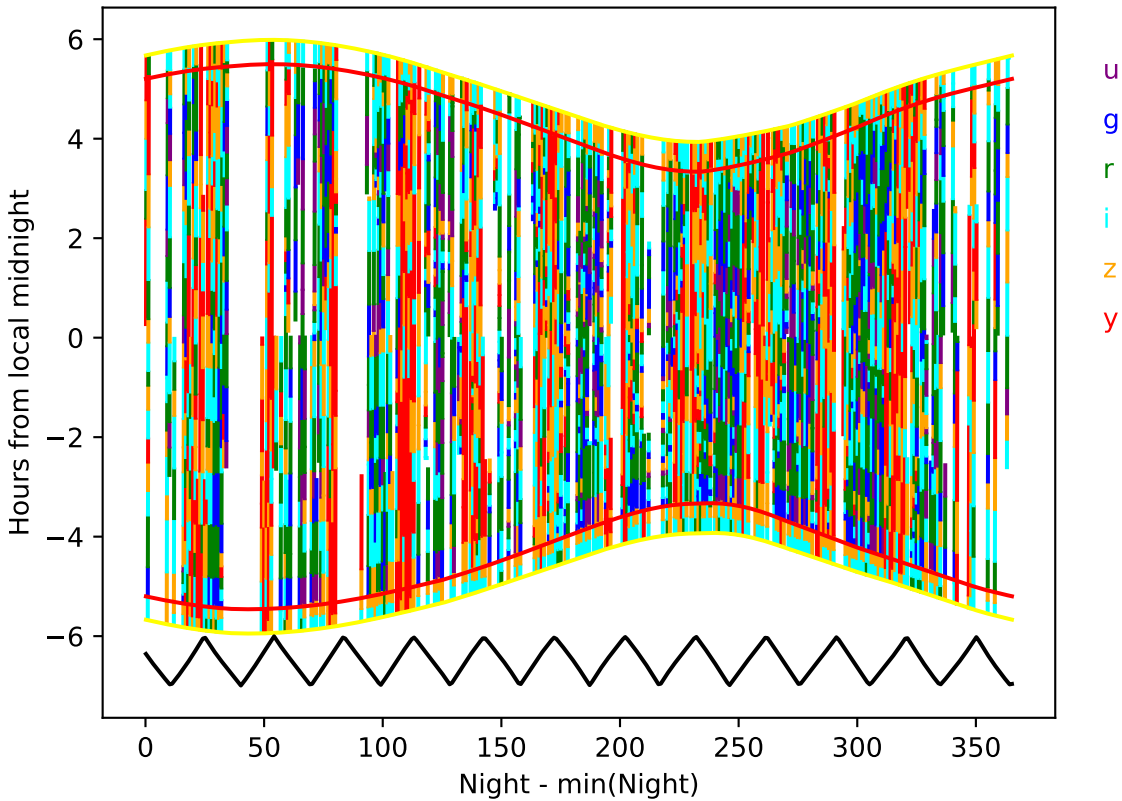
ddf_acor_sf20_lsf40_lsr20_v3.4_10yrs year 4-5: Hourglass
