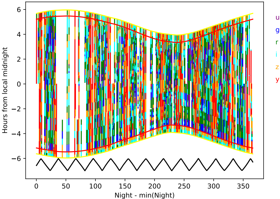
ddf_acor_sf20_lsf40_lsr20_v3.4_10yrs year 3-4: Hourglass
