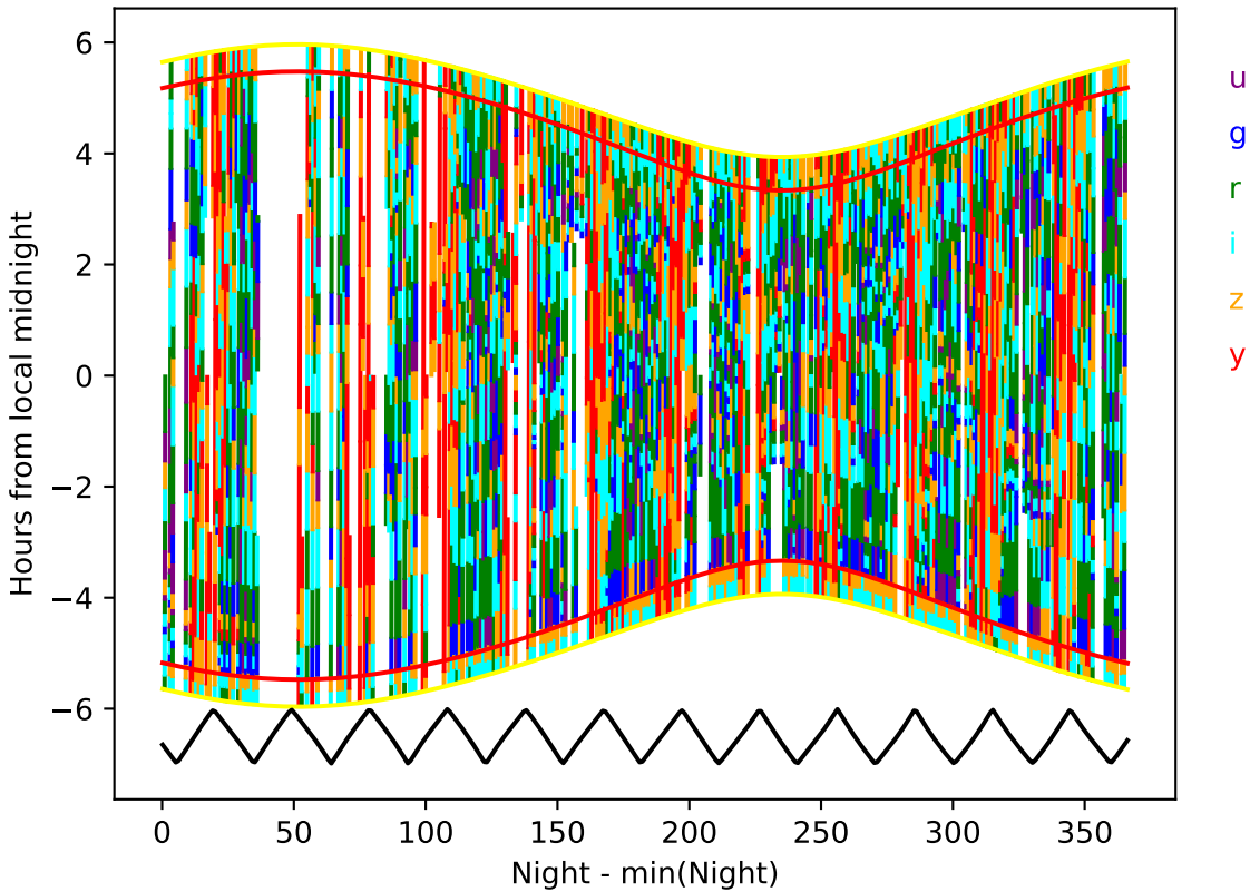
ddf_acor_sf20_lsf40_lsr20_v3.4_10yrs year 2-3: Hourglass
