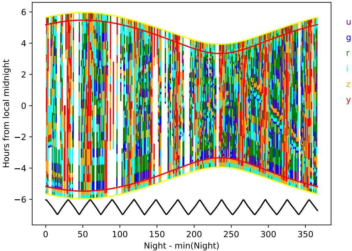
ddf_acor_sf20_lsf40_lsr20_v3.4_10yrs year 1-2: Hourglass
