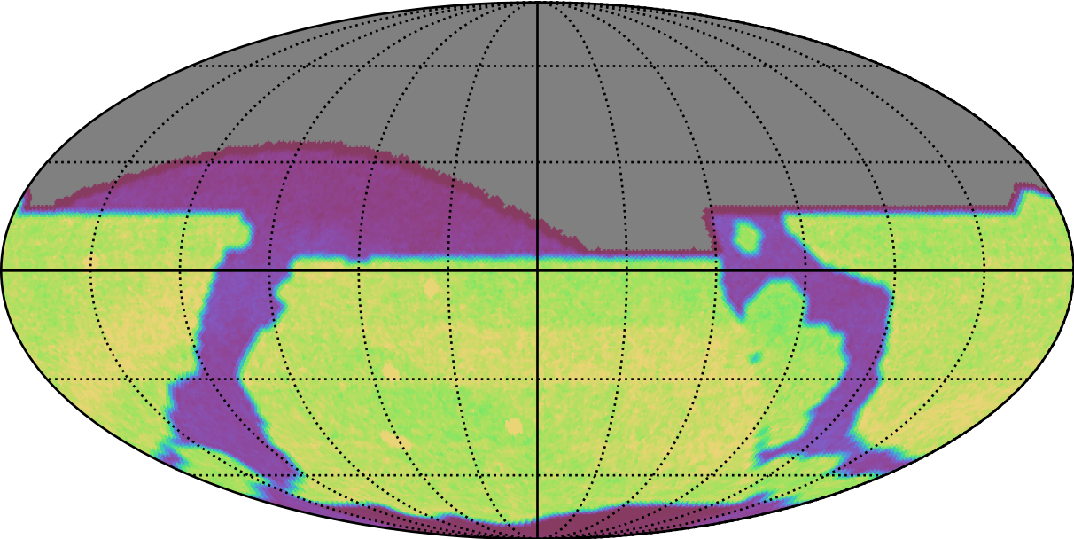
ddf_acor_sf20_lsf40_lsr20_v3.4_10yrs : Count observationStartMJD
