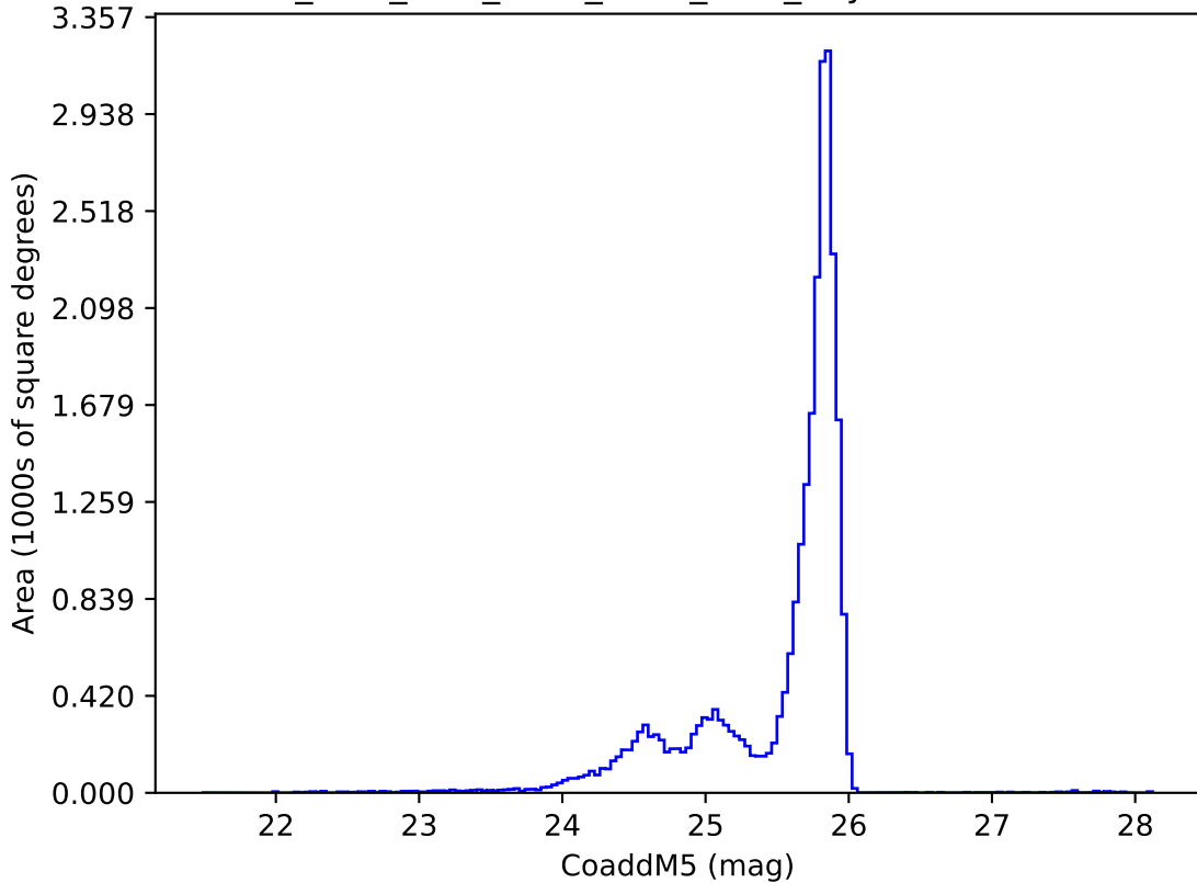
ddf_acor_sf20_lsf40_lsr20_v3.4_10yrs z: CoaddM5
