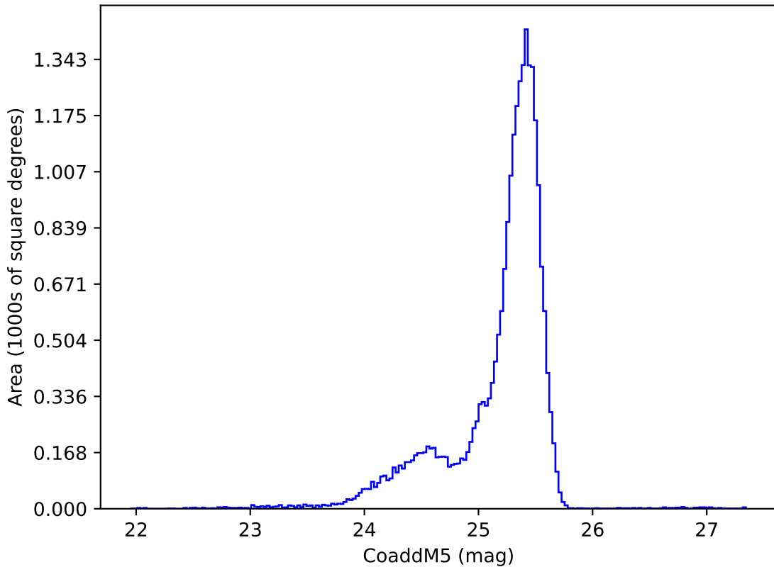
ddf_acor_sf20_lsf40_lsr20_v3.4_10yrs u: CoaddM5
