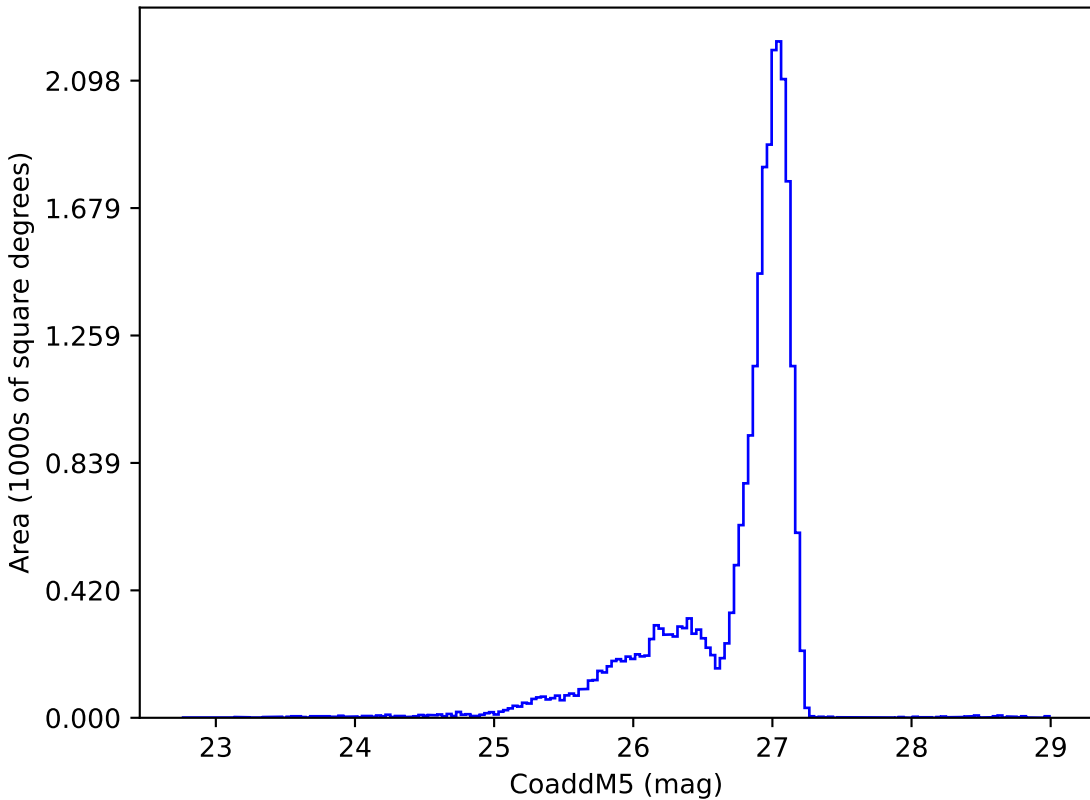
ddf_acor_sf20_lsf40_lsr20_v3.4_10yrs r: CoaddM5
