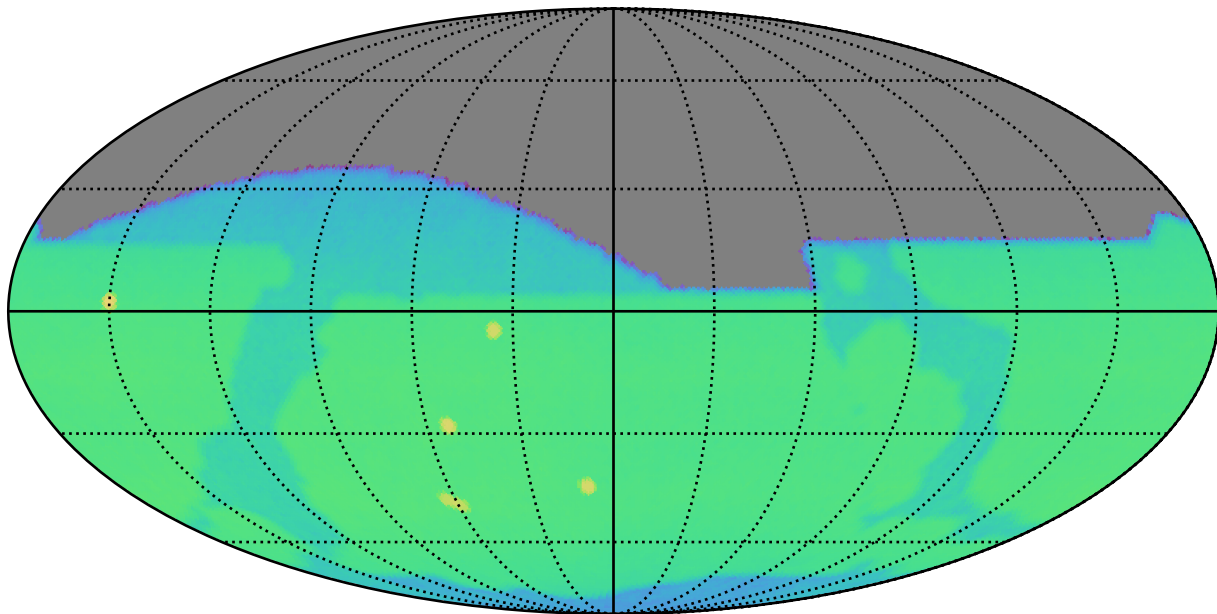
ddf_acor_sf20_lsf40_lsr20_v3.4_10yrs i: CoaddM5
