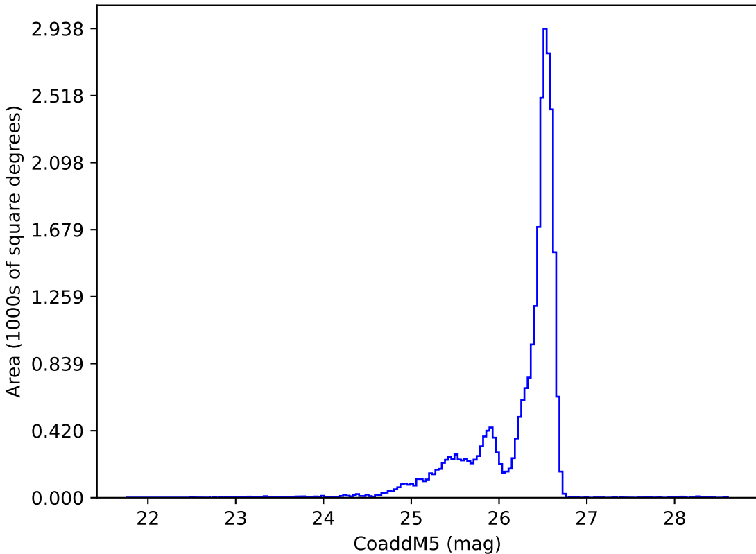
ddf_acor_sf20_lsf40_lsr20_v3.4_10yrs i: CoaddM5
