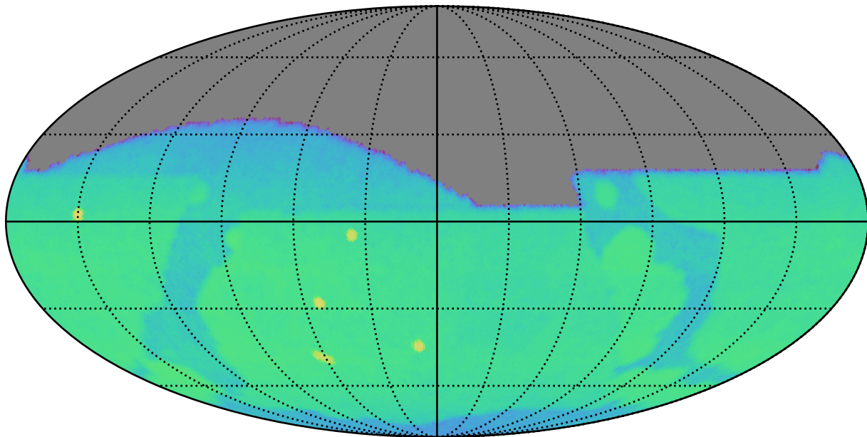
ddf_acor_sf20_lsf40_lsr20_v3.4_10yrs g: CoaddM5
