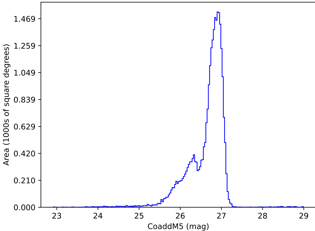
ddf_acor_sf20_lsf40_lsr20_v3.4_10yrs g: CoaddM5
