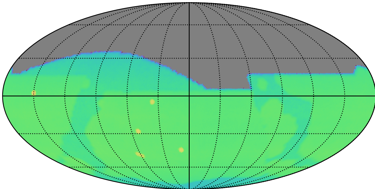
ddf_acor_sf20_lsf40_lsr20_v3.4_10yrs : CoaddM5
