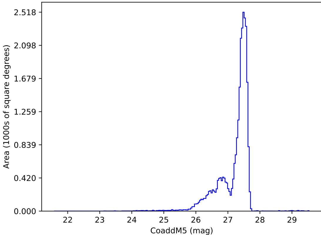
ddf_acor_sf20_lsf40_lsr20_v3.4_10yrs : CoaddM5
