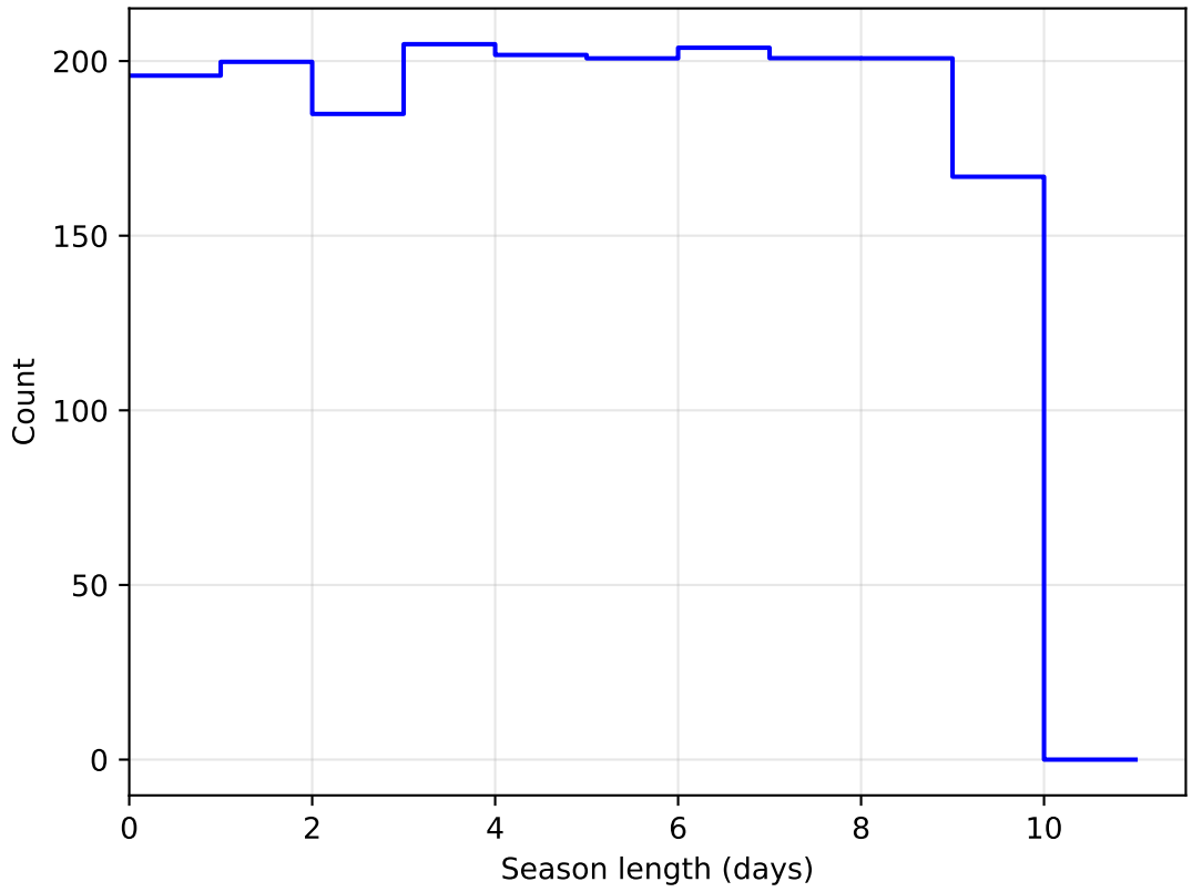
ddf_acor_sf20_lsf40_lsr20_v3.4_10yrs DD:ECDFS all bands: SeasonLength
