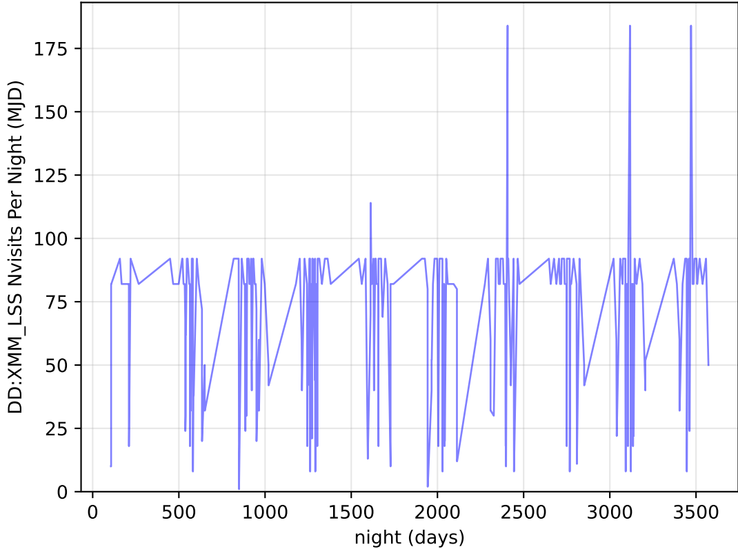
ddf_acor_sf20_lsf40_lsr20_v3.4_10yrs all bands: DD:XMM_LSS Nvisits Per Night
