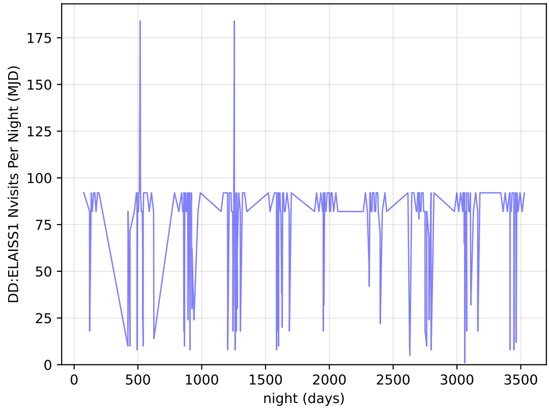
ddf_acor_sf20_lsf40_lsr20_v3.4_10yrs all bands: DD:ELAISS1 Nvisits Per Night
