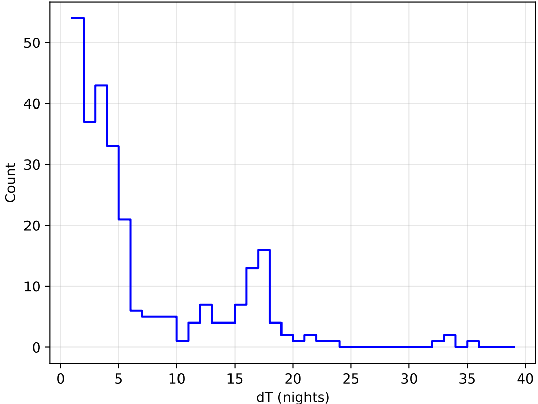
ddf_acor_sf20_lsf40_lsr20_v3.4_10yrs all bands: DD:ELAISS1 Delta Nights Histogram
