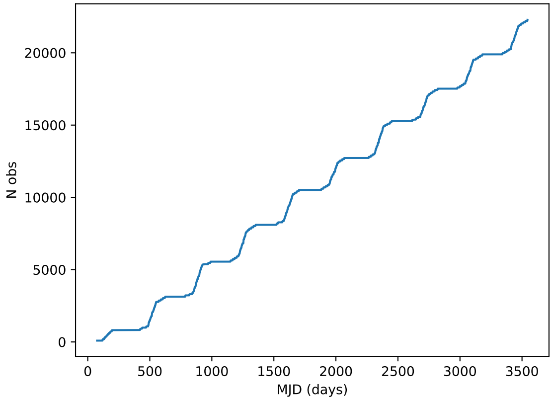
ddf_acor_sf20_lsf40_lsr20_v3.4_10yrs all bands: DD:ELAISS1 Cumulative NVisits
