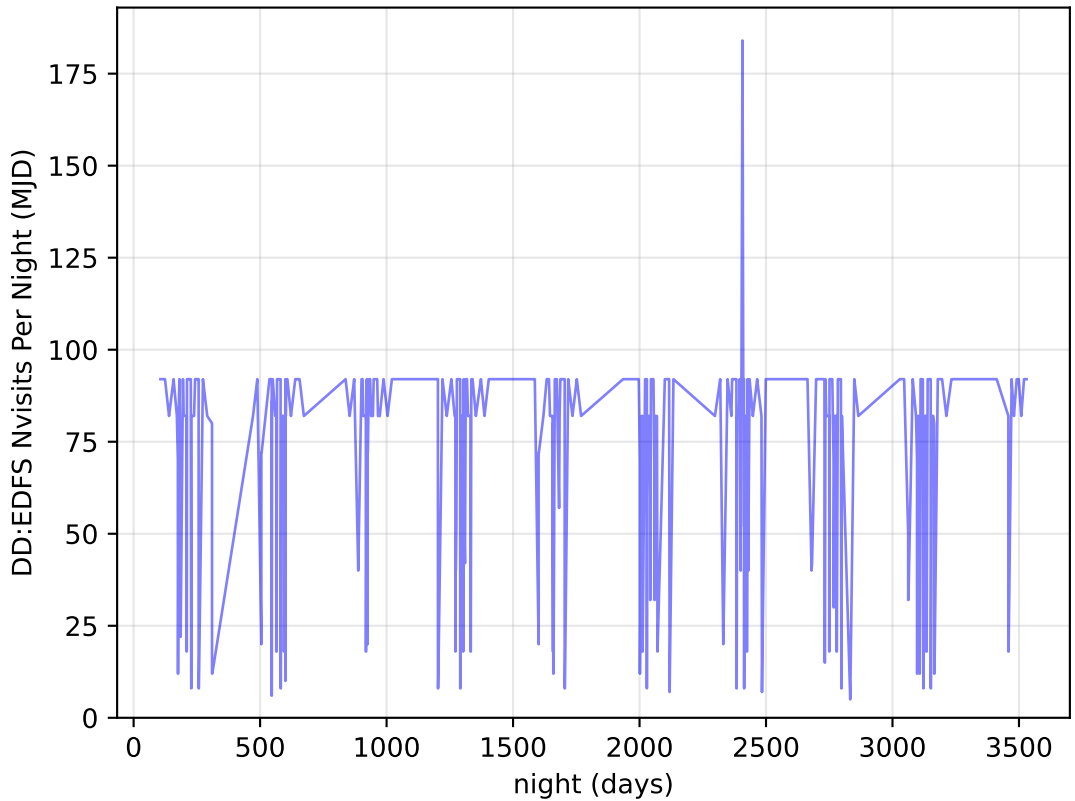
ddf_acor_sf20_lsf40_lsr20_v3.4_10yrs all bands: DD:EDFS Nvisits Per Night
