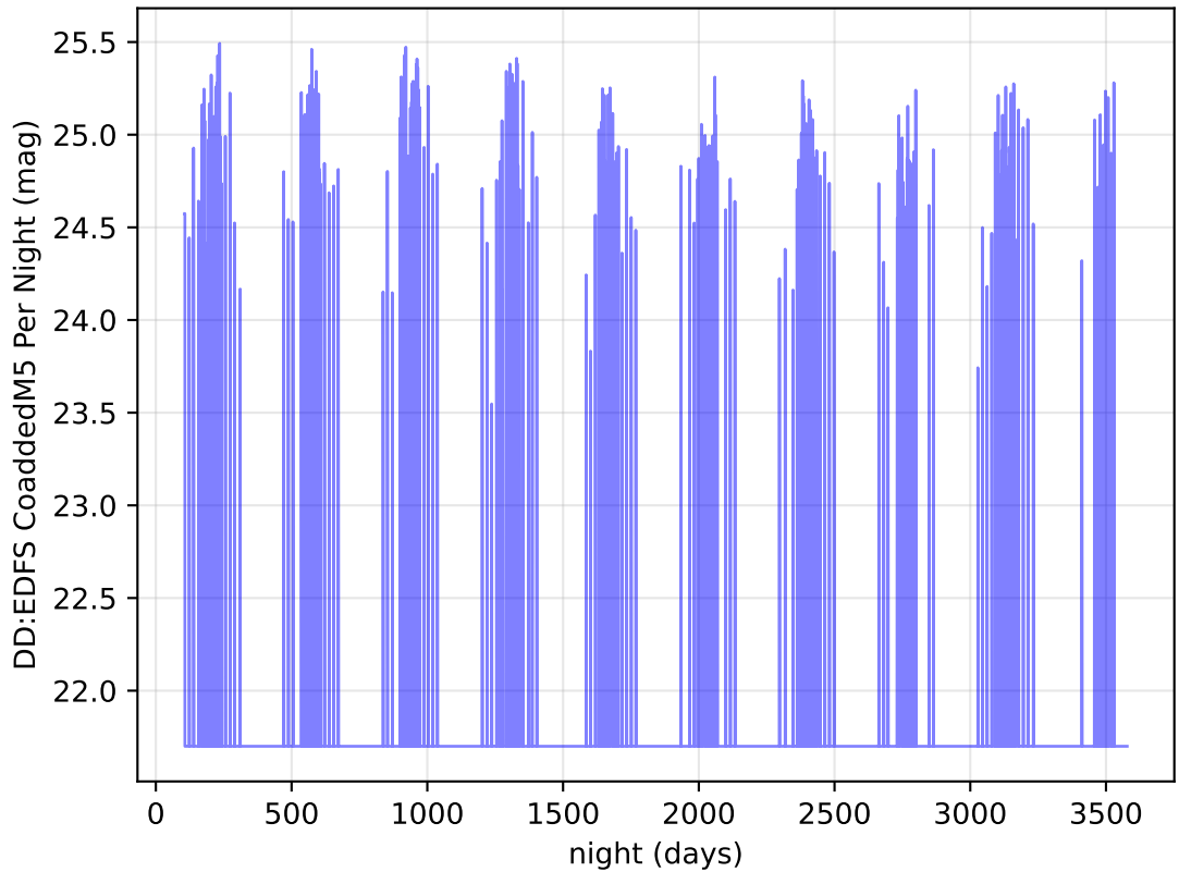
ddf_acor_sf20_lsf40_lsr20_v3.4_10yrs z band: DD:EDFS CoaddedM5 Per Night
