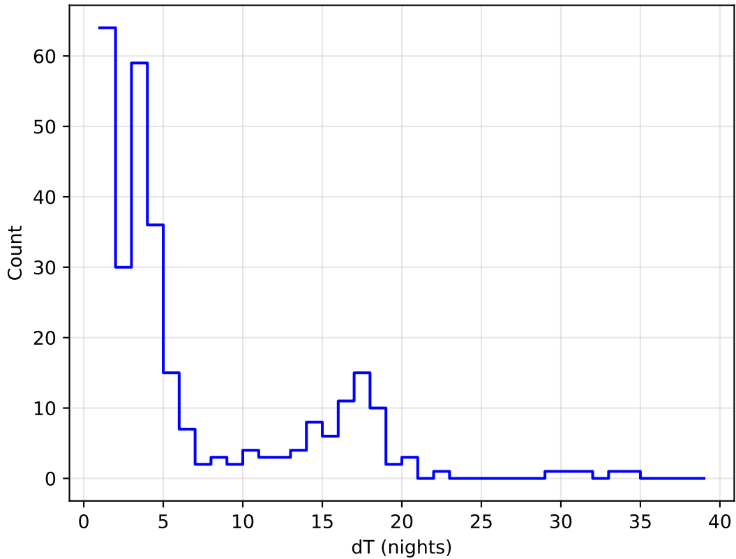
ddf_acor_sf20_lsf40_lsr20_v3.4_10yrs all bands: DD:ECDFS Delta Nights Histogram
